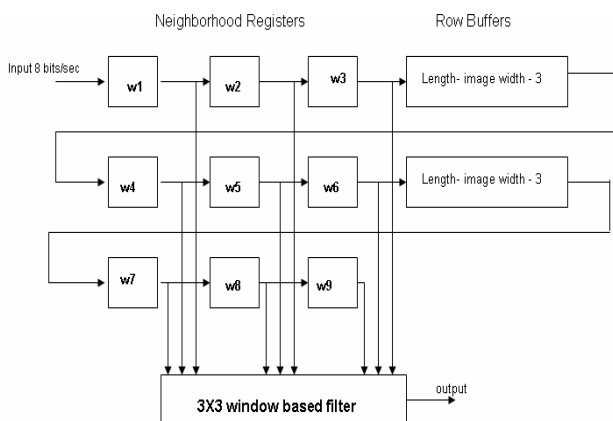
Fig.12. Implementation of a 3 \times 3 median filter window
