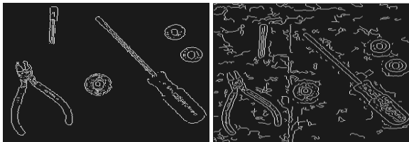
a) Sobel mask method b) Canny mask method Fig.14. Edge-detection
